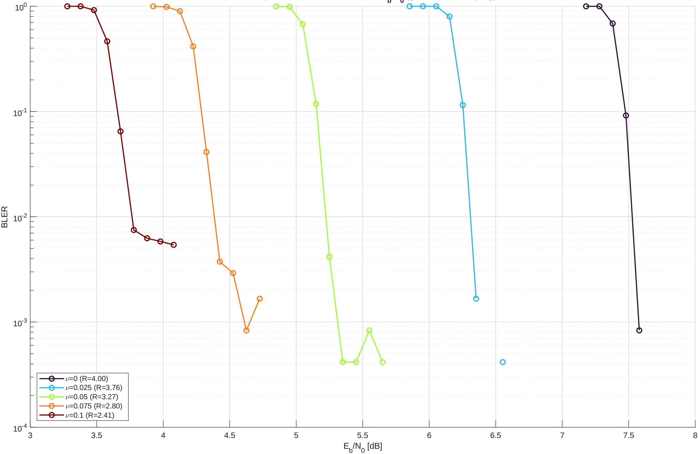
PAS 64-QAM, DVB-S2 2/3 — BLER vs E_b/N_0 (ganancia de shaping)
